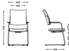
BELITE 5102 weight: 12,9 kg
