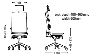
BELITE 3013 weight: 21,5 kg
