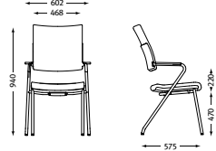
BELITE 7102 weight: 11,8 kg
