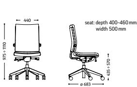
BELITE 1013 weight: 20,2 kg
