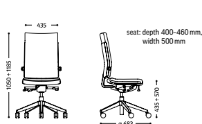
BELITE 2013 weight: 20,6 kg
